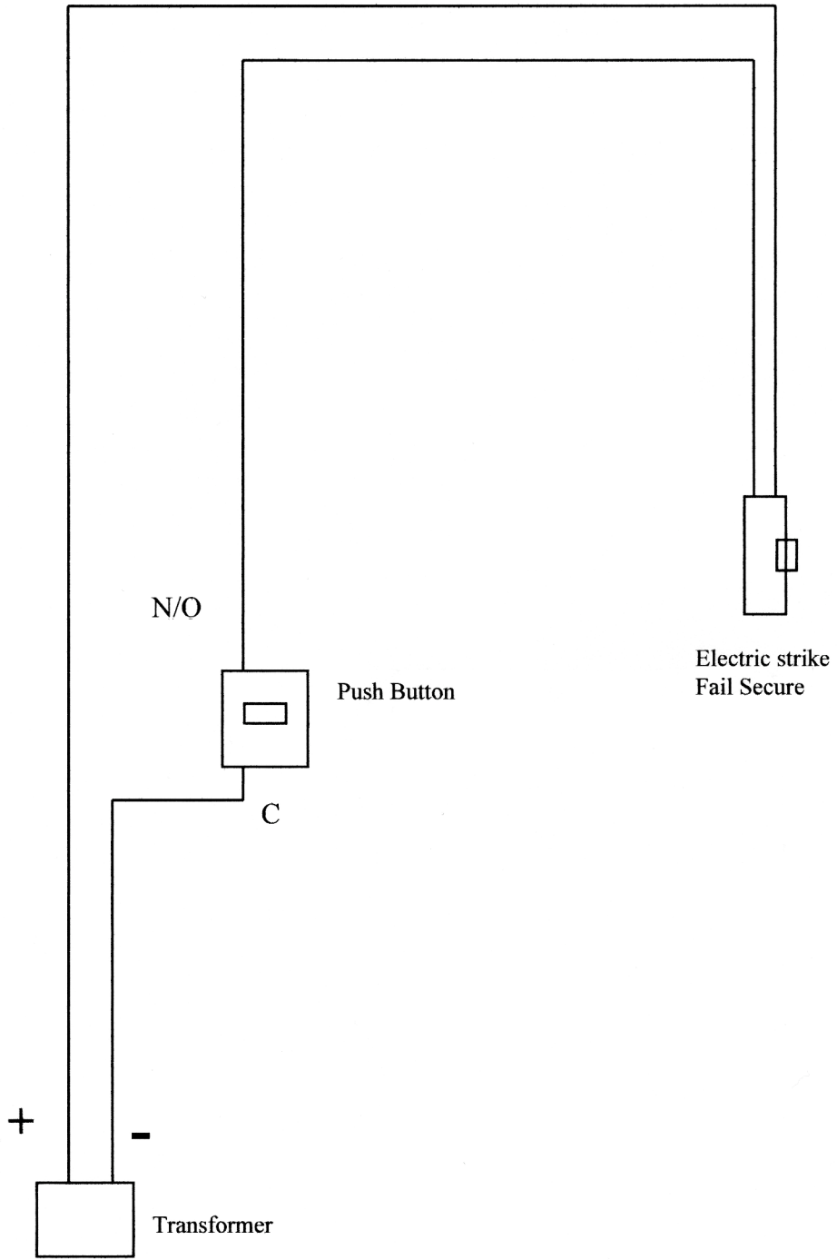
Wiring diagram # 1
